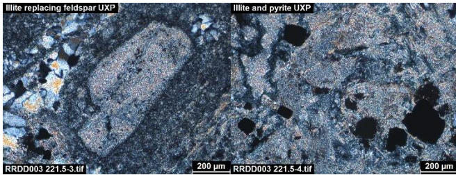
Photomicrographs for RRDD003 221.5
