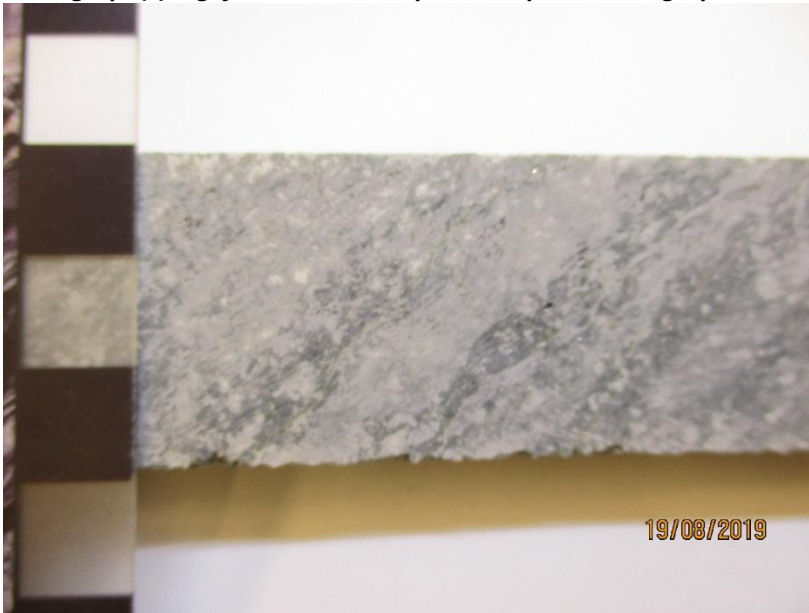
HAND-SPECIMEN IMAGE OF RRDD003 - 221.55
